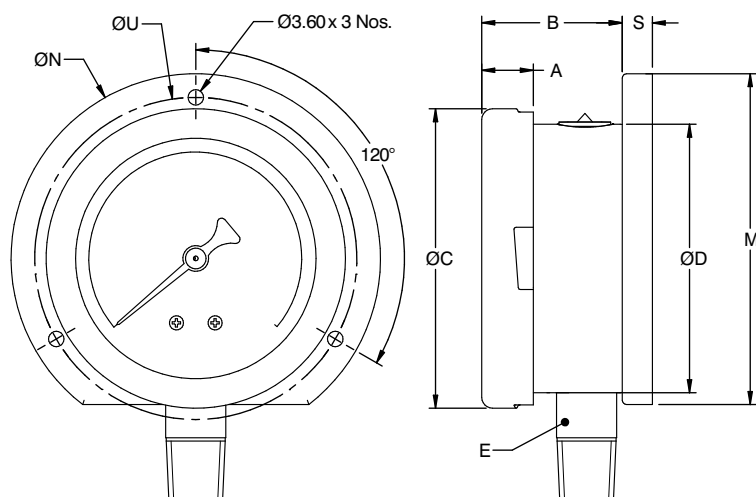
Type B1 (Bayonet ring)
