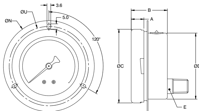
Type L1 (Bayonet ring)
