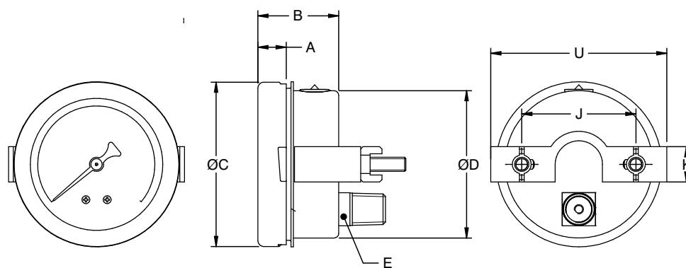
Type L2 (Bayonet ring)
