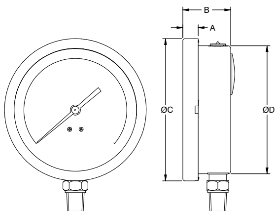
Type B0 (Bayonet ring)
