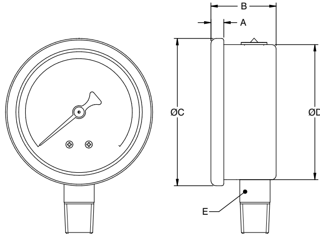
Type B0 (Rolling ring)
